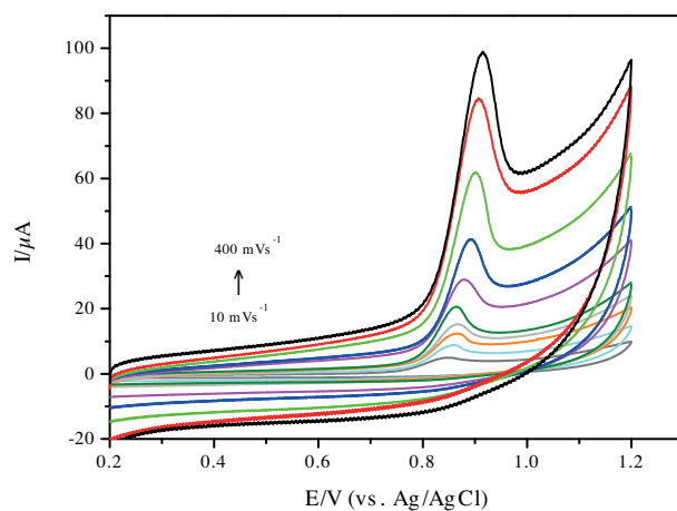
Figure S1. Cyclic voltammograms of 10 \mu M CEF at IL/Bi-film/PGE with different scan rates. Curves from bottom to top are obtained at 10, 20, 30, 40, 60, 80, 150, 200, 300, and 400 mV s -1 , respectively. Conditions: pH 4.0 BR; Ei: 0.2 V; Ef: 1.2 V.
