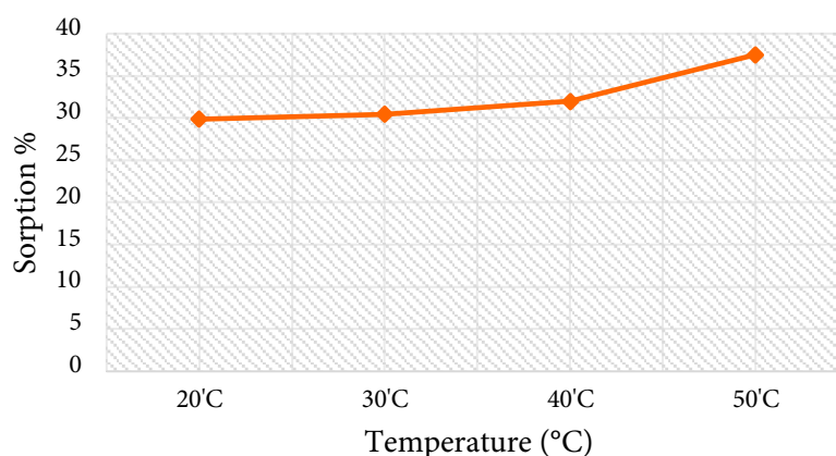
Figure 4. The effect of temperature on P sorption ( C_0 ; 100\text{ mg L}^{-1} , shaking time; 4 h, sorbent amount; 1\text{ g} / 30\text{ mL} , particle size; 0.42\text{ mm} , \text{pH} = 6.12 ).
