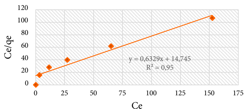
Figure 7. Phosphorus sorption of gyttja according to the Langmuir isotherm (Sorbent amount; 1 g / 30 ml, temperature; 21 \pm 2 °C, particle size; 0.42 mm, shaking time; 12 hours, pH; 6.12)
