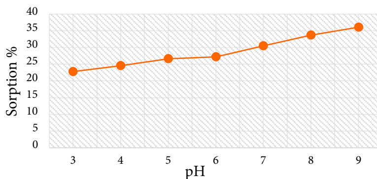
Figure 3. The effect of pH on P sorption ( C_0 ; 100 \text{ mg L}^{-1} , shaking time; 4 h, amount of sorbent; 1 \text{ g} / 30 \text{ mL} , temperature; 21 \pm 2 \text{ }^\circ\text{C} , particle size; 0.42 mm)
