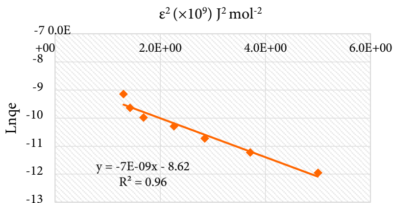
Figure 8. Evaluation of P sorption by gytja with D-R isotherm (Sorbent amount; 1 g / 30 mL, temperature; 21 ± 2 °C, particle size; 0.42 mm, shaking time; 12 h, pH = 6.12)
