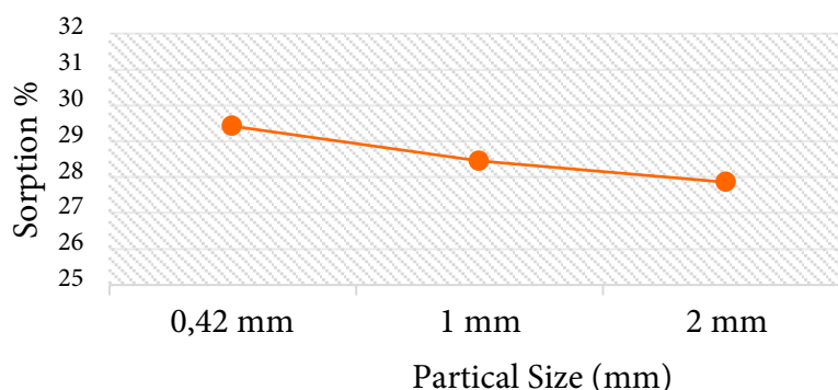
Figure 2. The effect of particle size on P sorption ( C_0 ; 100 \text{ mg L}^{-1} , shaking time; 4 hours, amount of sorbent; 1 \text{ g} / 30 \text{ mL} , temperature; 21 \pm 2 \text{ }^\circ\text{C} , pH = 6.12)
