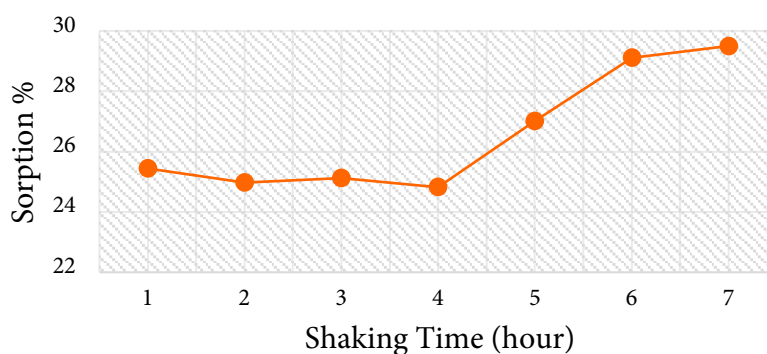
Figure 5. The effect of shaking time on P sorption ( C_0 ; 100\text{ mg L}^{-1} , sorbent amount; 1\text{ g} / 30\text{ mL} , temperature; 21 \pm 2^\circ\text{C} , particle size; 0.42\text{ mm} , \text{pH} = 6.12 ).
