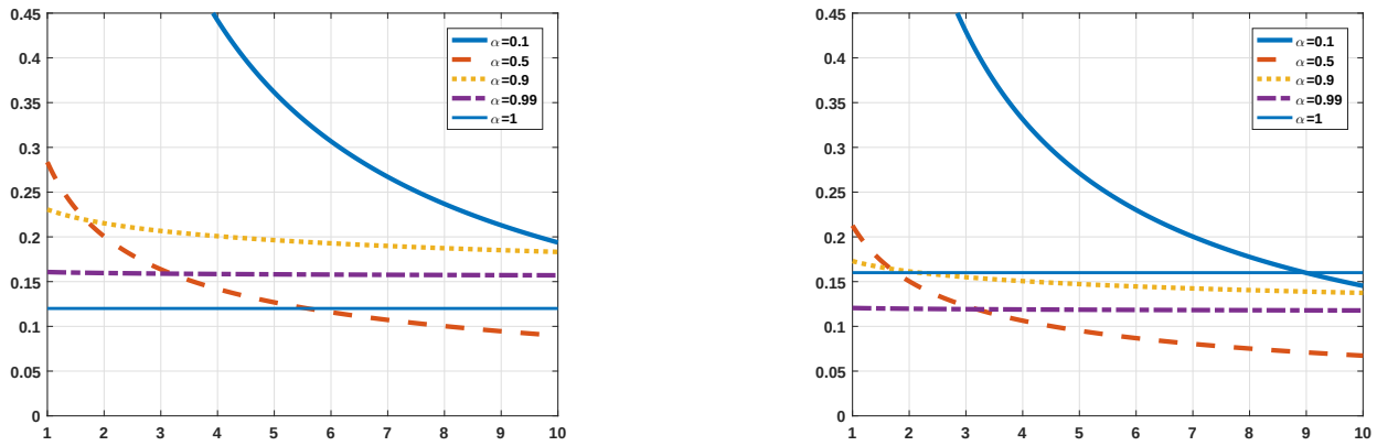
Figure 3. Graphs of \kappa_\alpha(s) = \frac{3\Gamma(2-\alpha)s^{\alpha-1}}{25\alpha} (left-hand side) and \tau_\alpha(s) = \frac{4\Gamma(2-\alpha)s^{\alpha-1}}{25\alpha} (right-hand side) for \alpha \in \{0.1, 0.5, 0.9, 0.99, 1\} .
