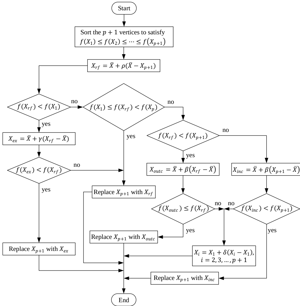
Figure 2. Flowchart of NM method
