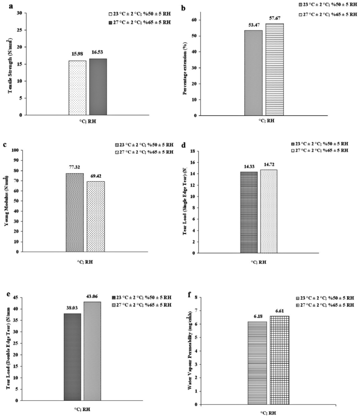
Figure 1: Changings in different atmospheric conditions (a: tensile strength, b: percentage extension, c: Young's modulus, d: single edge tear load, e: double edge tear load, f: water vapour permeability). Results are the means of sixty replicates samples \pm SD.
