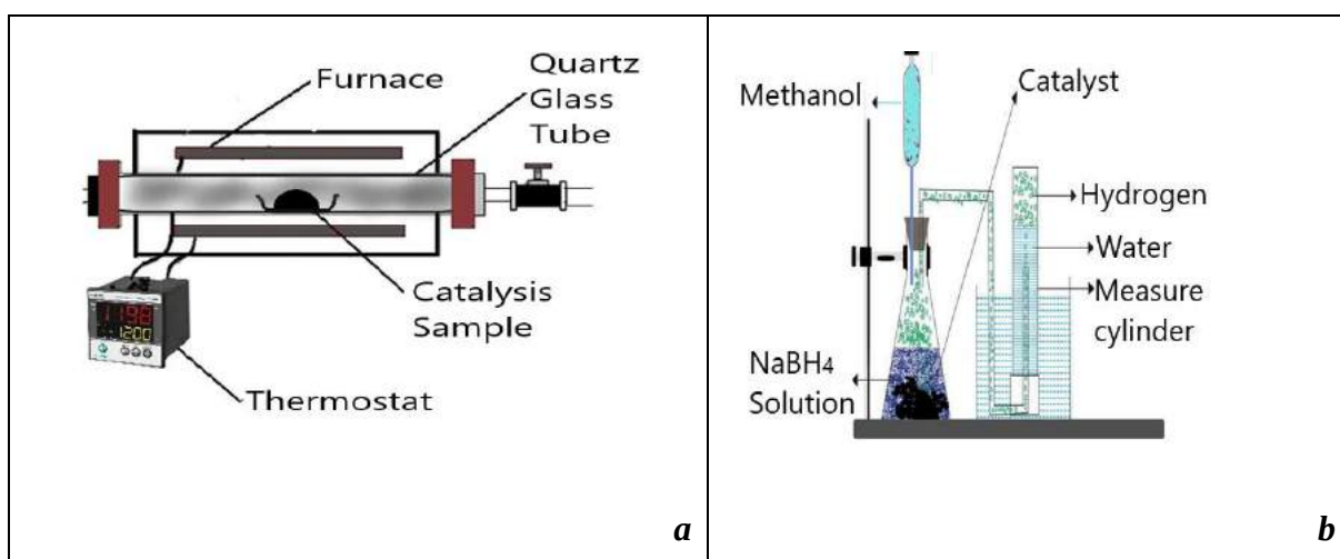
Fig 2. Furnace System Scheme for Catalyst Preparation (a) Hydrogen Gas Measurement Scheme (b)
