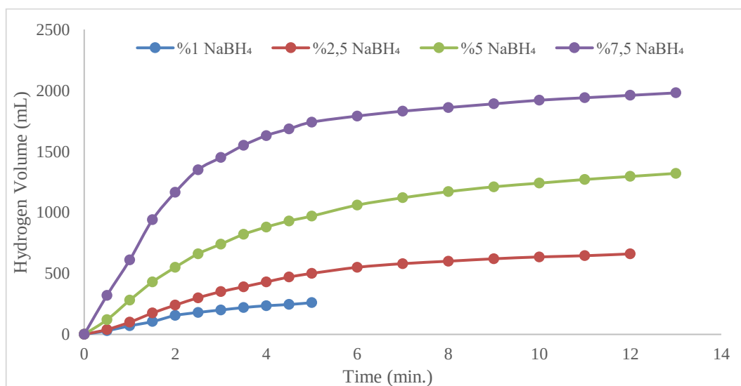
Fig 6. Investigation of the effect of different sodium boron hydride concentrations on the hydrogen production rate in the presence of \text{Al}_2\text{O}_3/\text{Spirulina Platensis} supported Co catalysts ( w_{\text{cat}}=0,1\text{ g} , T=30^\circ\text{C} , V_{\text{solution}}=10\text{ mL} )
