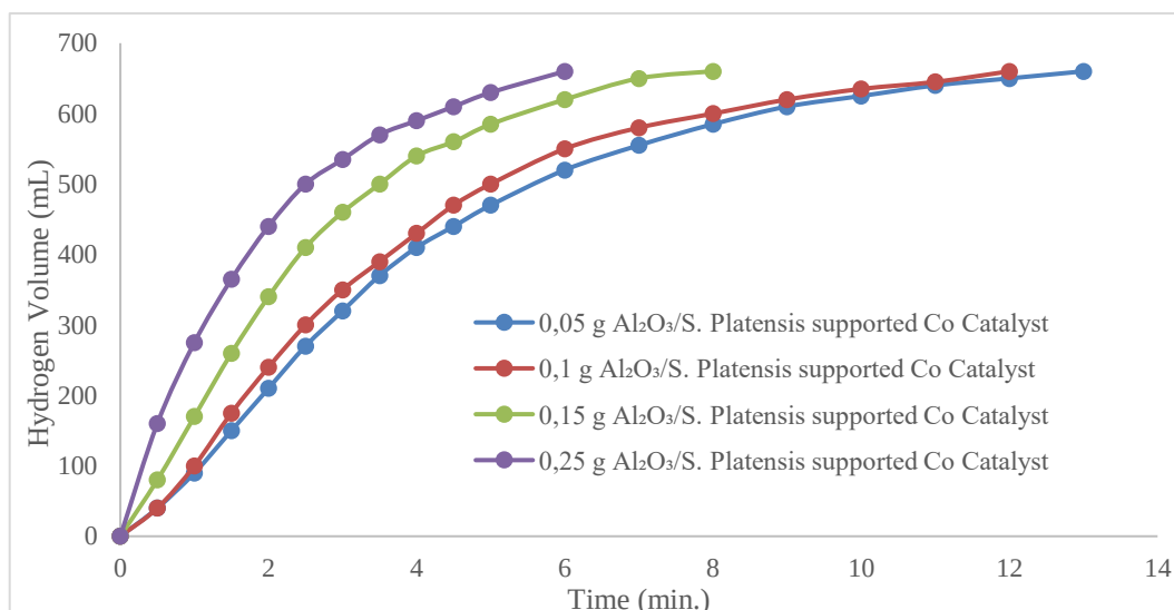
Fig 5. The effect of different amounts of \text{Al}_2\text{O}_3/\text{Spirulina Platensis} supported Co catalyst on the degradation of sodium borohydride (% 2,5 \text{NaBH}_4 , T=30^\circ\text{C} , V_{\text{solution}}=10\text{ mL} )
