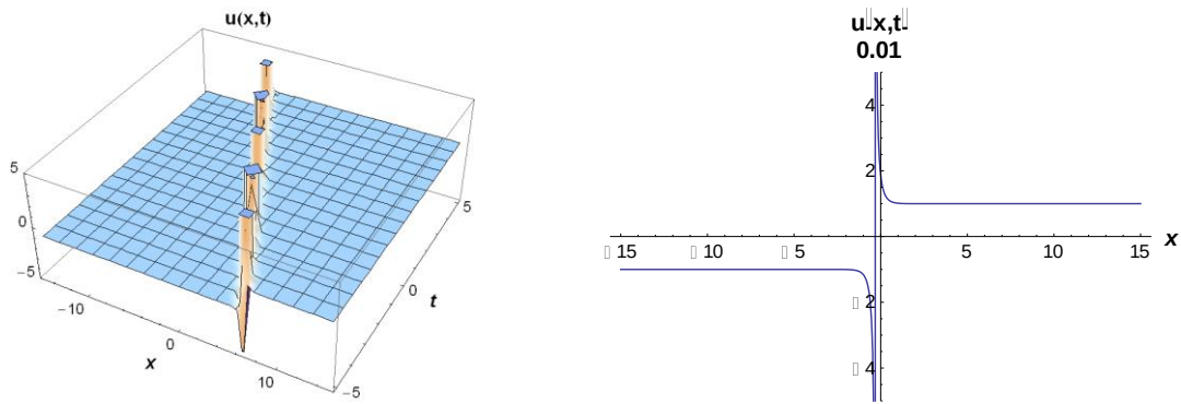
Figure 1. The 3D and 2D surfaces of Eq. (23) for \lambda = 0.3, \mu = -0.2, k = 4, a = 2, E = 0.5, -15 < x < 15, -5 < t < 5 and t = 0.01 for 2D surface.
