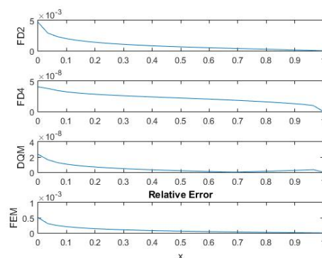
Figure 2. Comparison of relative error in Problem 1 for N=30
