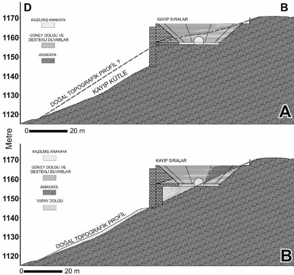
Fig. 25 The real scaled topographic profile of the hill where the stadium located and the situation of the southern seat rows.
