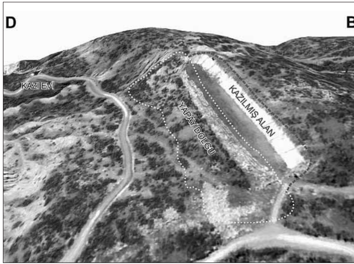
Fig. 24 The combination of the satellite image and digital elevation model of the stadium and the approximate situations of excavated and artificial fill areas (Elitez – Yaltırak 2012).
