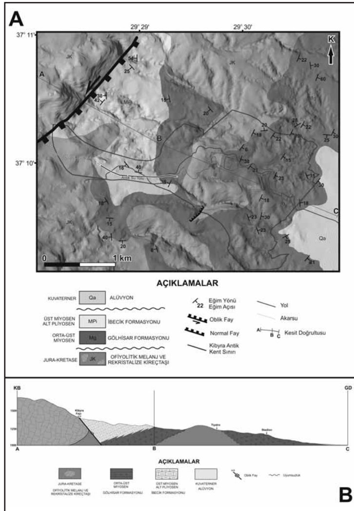
Fig. 23 The geological map (A) and cross-section (B) of Kibyra (Elitez – Yaltırak 2012)
