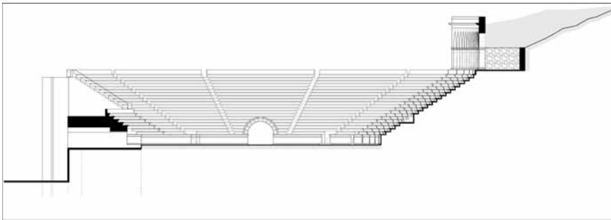
Fig. 7 Cross-section of 21 rows of seats extending to end of sphendone arch (Architects I. Akgül – N. Gürlesin – M. Sayan – N. Kocaman).
