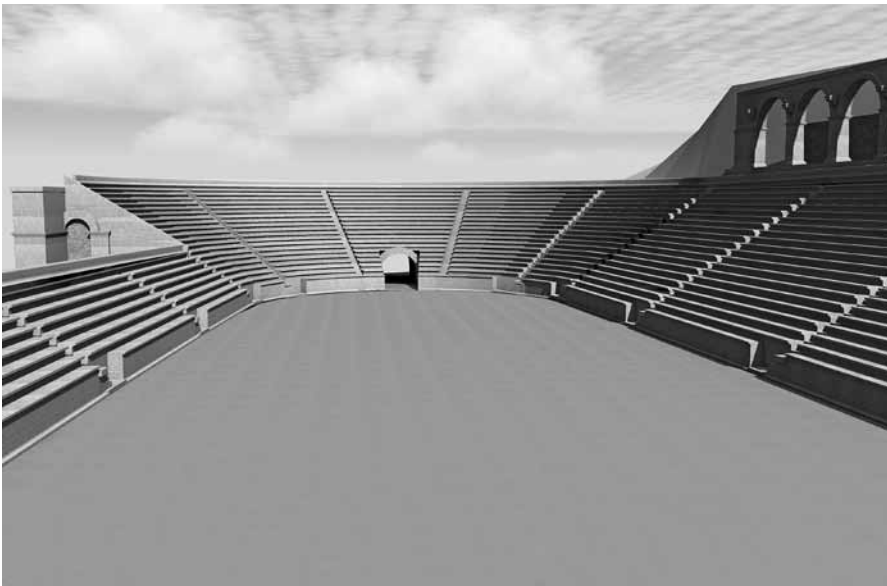
Fig. 8 3-D View of 21 rows of seats extending to end of sphendone arch (Architects I. Akgül – N. Gürlesin – M. Sayan – N. Kocaman).
