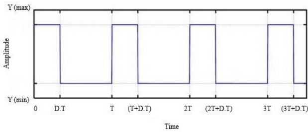
Figure 2. PWM wave ymin, ymax and D parameters
