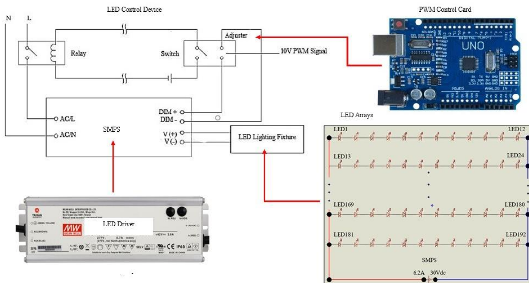
Figure 4. Block schematic form of the light level control
