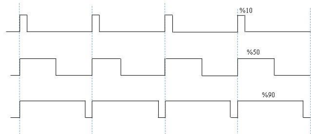
Figure 3. PWM ratios determining the light level
