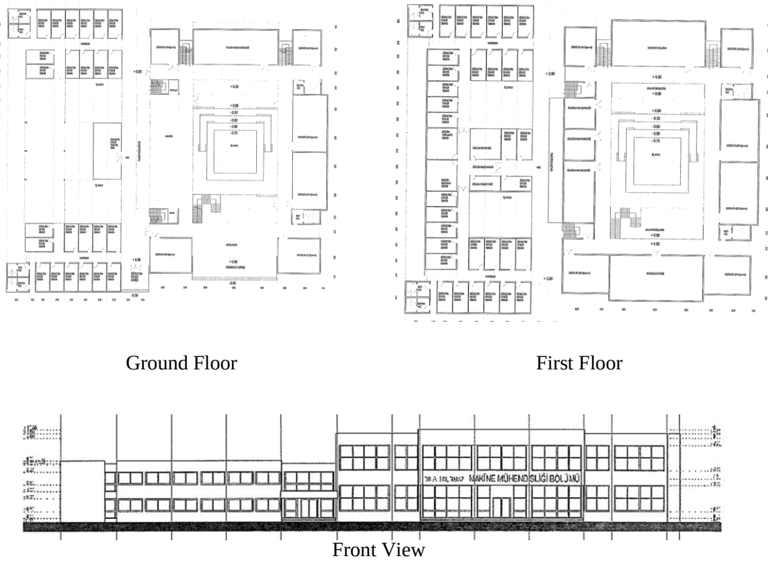
Figure 3. Mechanical Engineering Department view and plans
