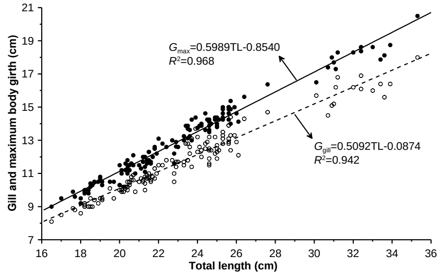
Figure 1. Total length-head girth and total length-maximum girth relationships of the bluefish ( Pomatomus saltatrix ) (● and ○: TL-G max ; ○ and ○: TL-G gill ).
