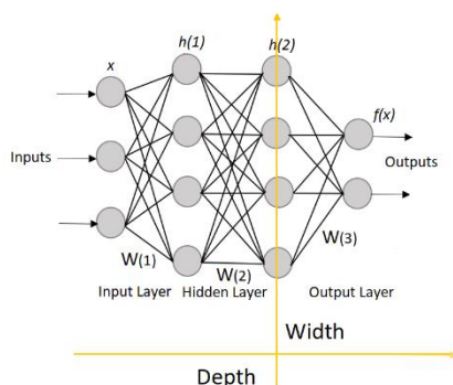
Figure 1. General structure of Multilayer Perceptron models [15]
