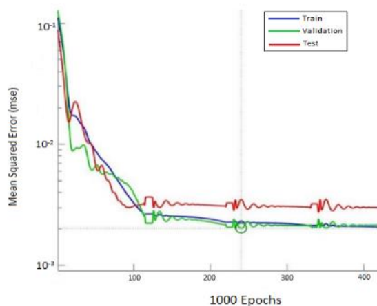
Figure 4. Decreasing MSE performance graph by number of training epochs
