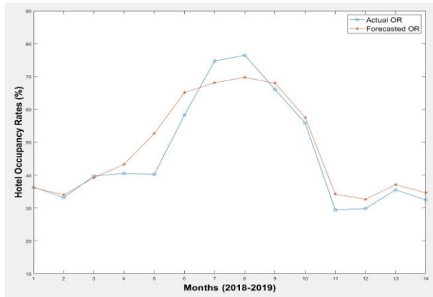
Figure 3. The graph of actual hotel OR data and forecasted OR data (Table 3. graph)
