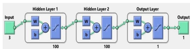
Figure 2. Designed MLP model
