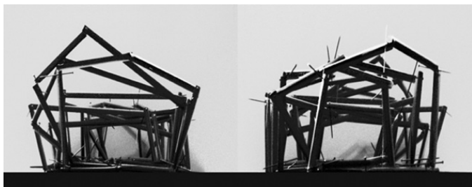
Figure 8. Perspective view, front and back elevations of the physical models of frames.
