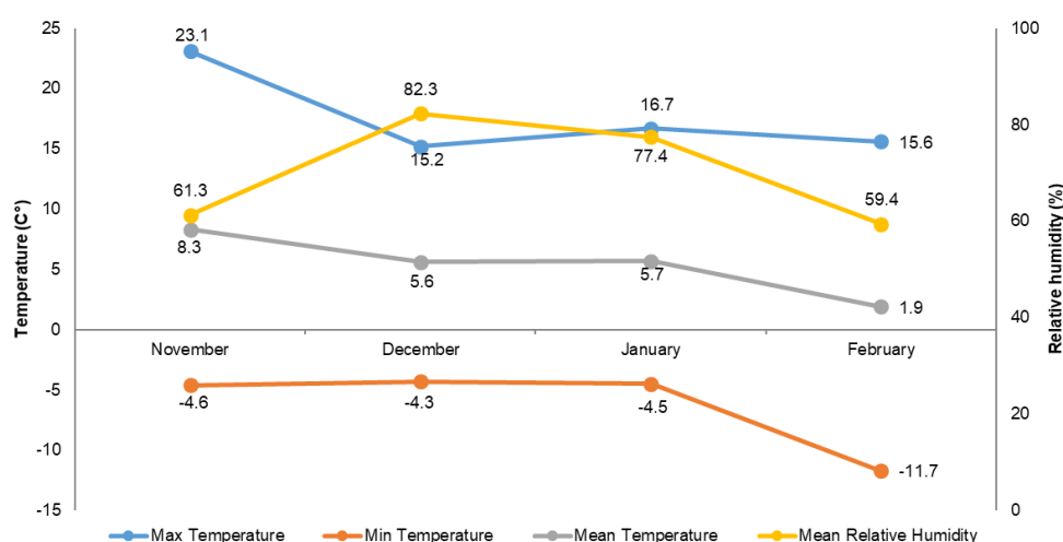
Figure 1. Monthly temperature and relative humidity variation in Korkuteli.
