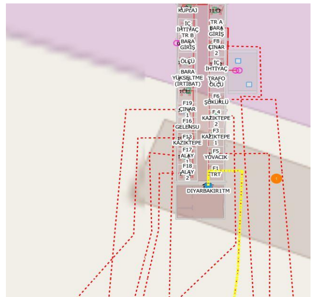
Figure 3. Feeder supplying the neighborhood
